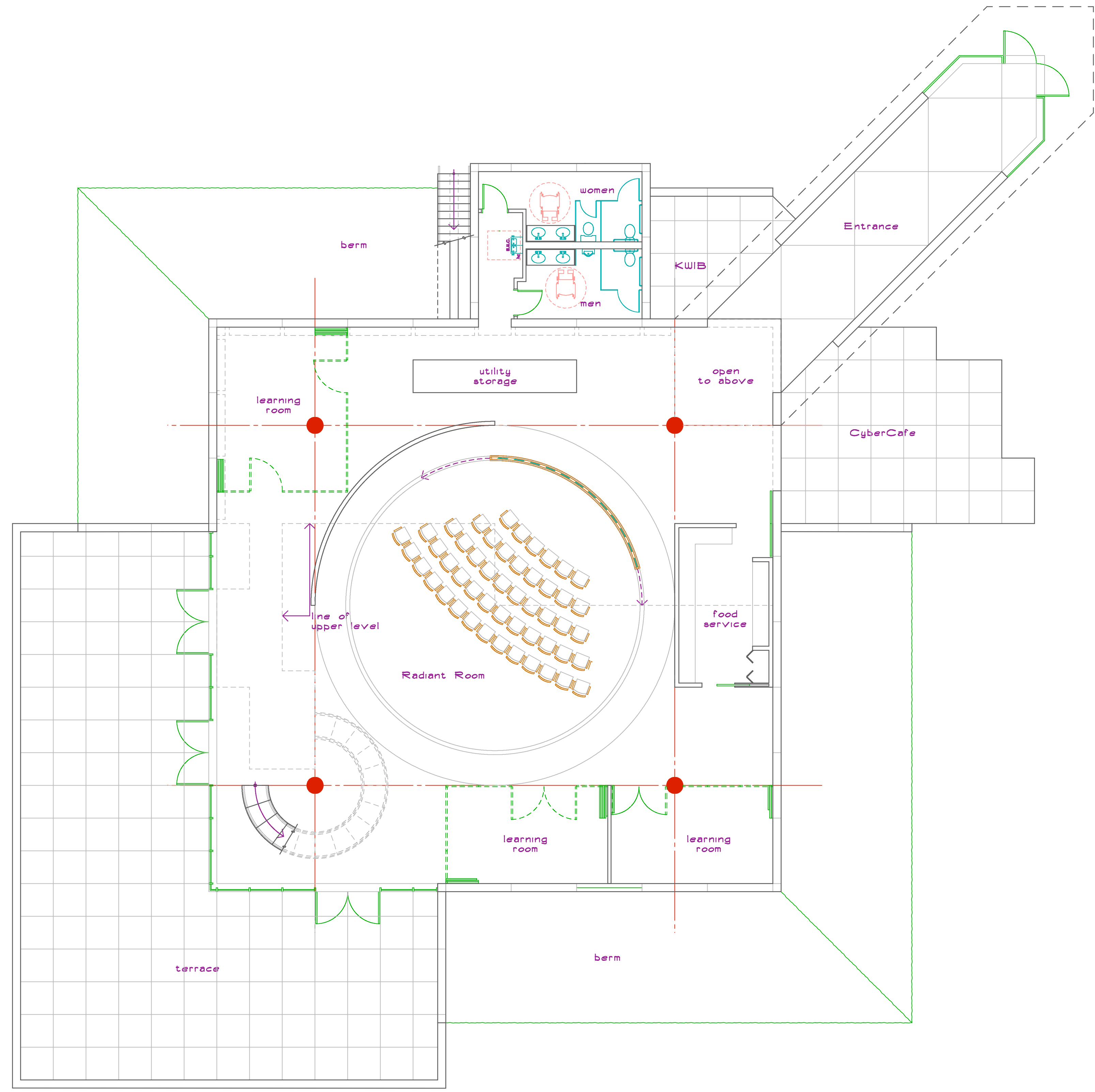
navCenter Pavilion Lower Floor Plan scale 1/8" = 1'-0"
